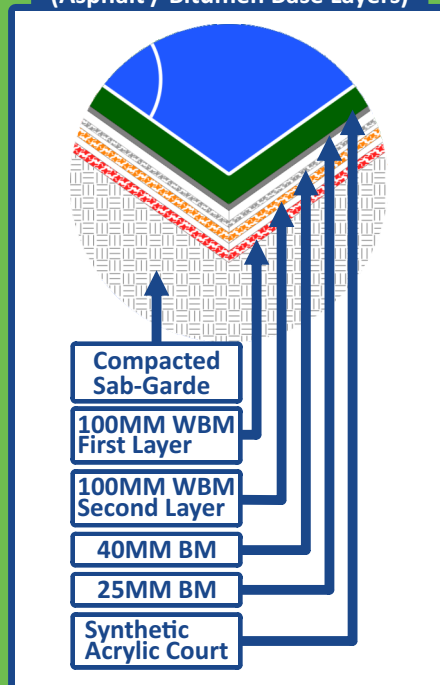
Detail-B (Acrylic 5 - Layers)
